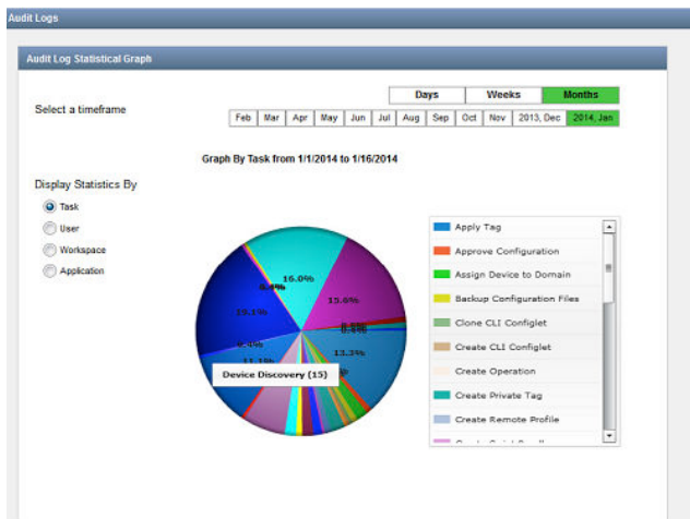
Figure 3: Audit Log
